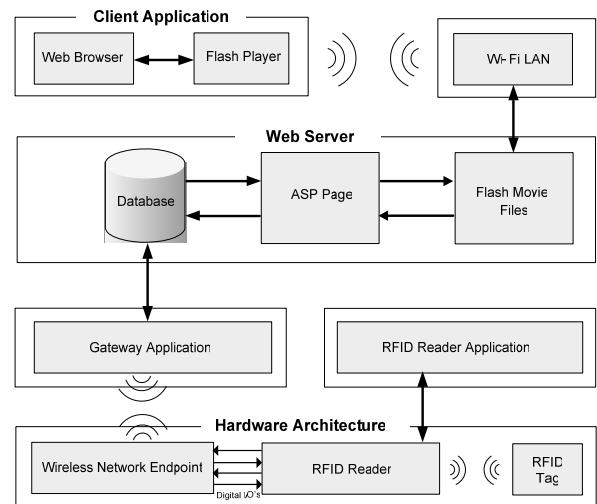
Fig.4 Communication Model
