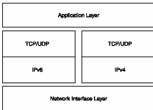
Fig1 Dual-Stack structure [7]
