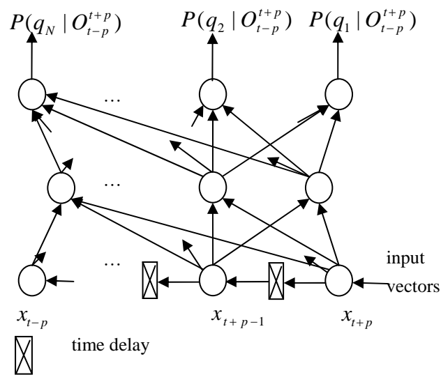
Figure 3. TDNN scheme for probability estimator
