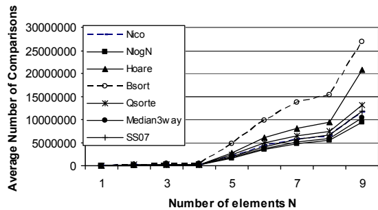
Fig. 6. Average Number of Comparisons for Random Data
