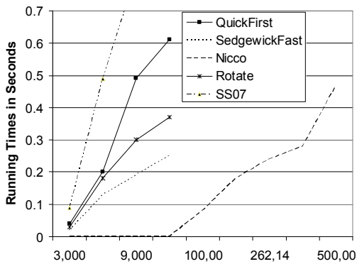
Fig. 10. Running times for Sorted Data
