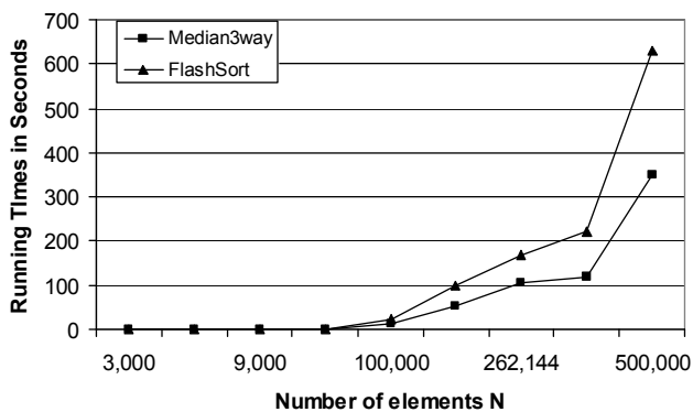
Fig. 3 Average Running Times for Random Data
