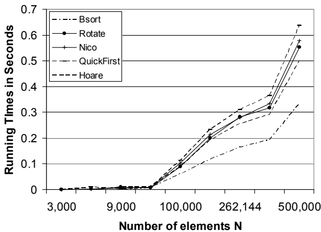
Fig. 2 Average Running Times for Random Data
