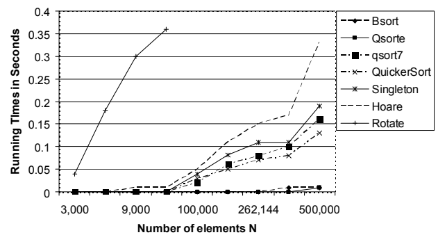
Fig. 12. Running times for Data Sorted in Reverse.
