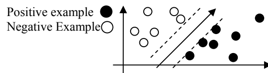
Fig. 2 Linear Support Vector Machine Classification
