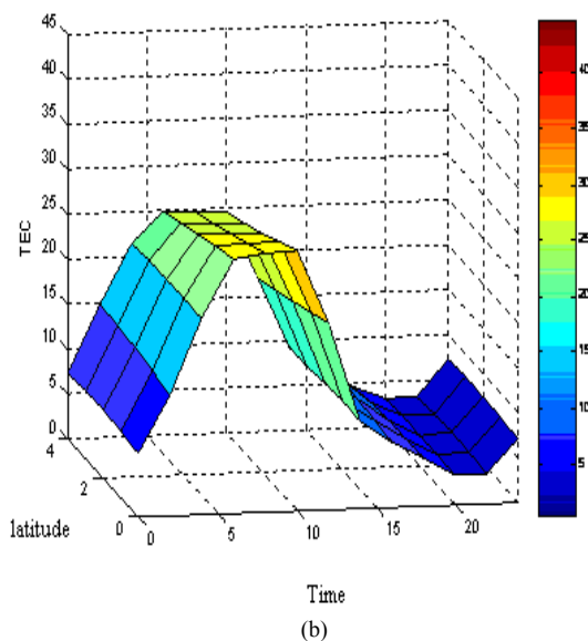
Fig. 7 (a) 3-D single layer model (SLM) for KTPK station (b) 3-D single layer model (SLM) for KUKP station
