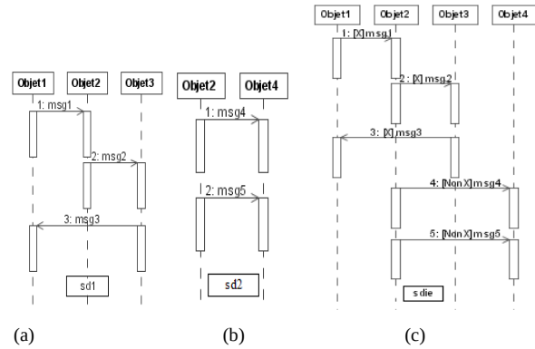
Fig. 12: (a) SequenceD sd1, (b) SequenceD sd2 et (c) Resulting SequenceD sdie = sd1 ? sd2.
