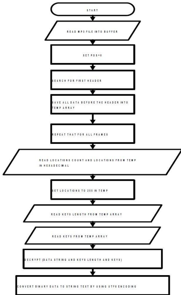
Fig.2. Flow Chart for extracting text of (BAF)
