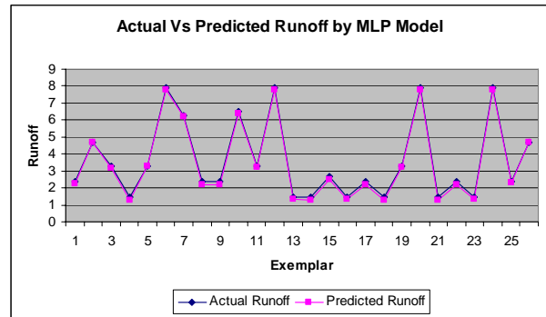
Figure 5- Actual Vs. Predicted runoff by MLP
