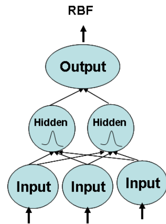
Figure 2. The Radial basis function neural network
