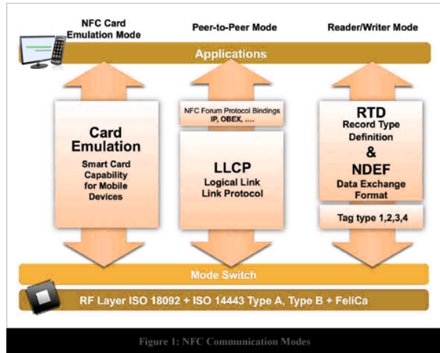
Figure 1: NFC Modes of Communication [19]
