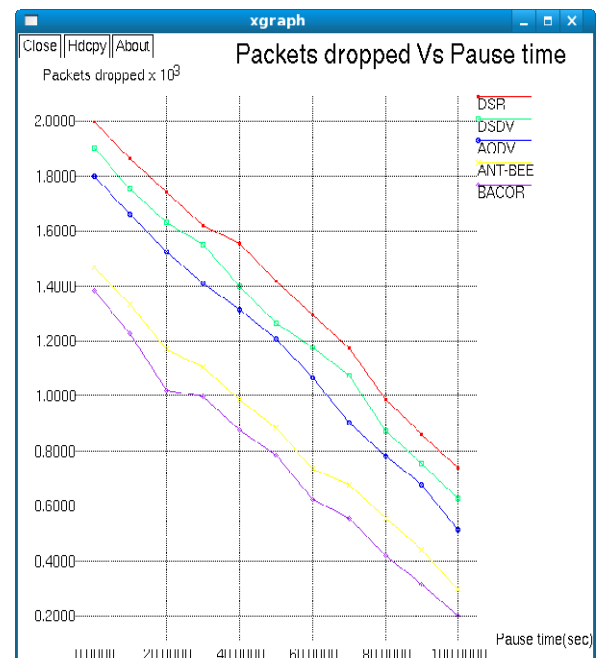
Figure6. Packets Dropped Vs Pause Time
