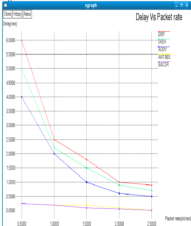
Figure3. Delay Vs Packet Rate
