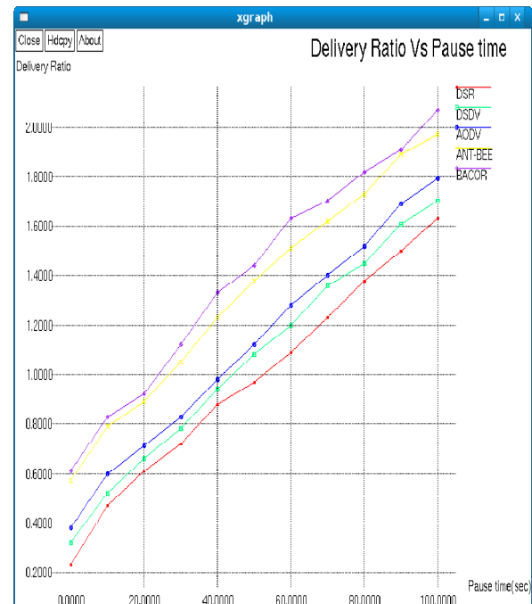
Figure2. Packet Delivery Ratio Vs Pause Time
