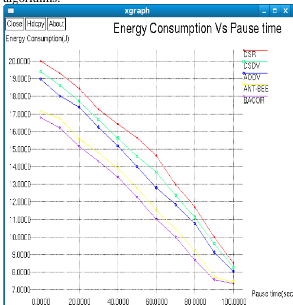
Figure4. Energy Consumption Vs Pause Time
