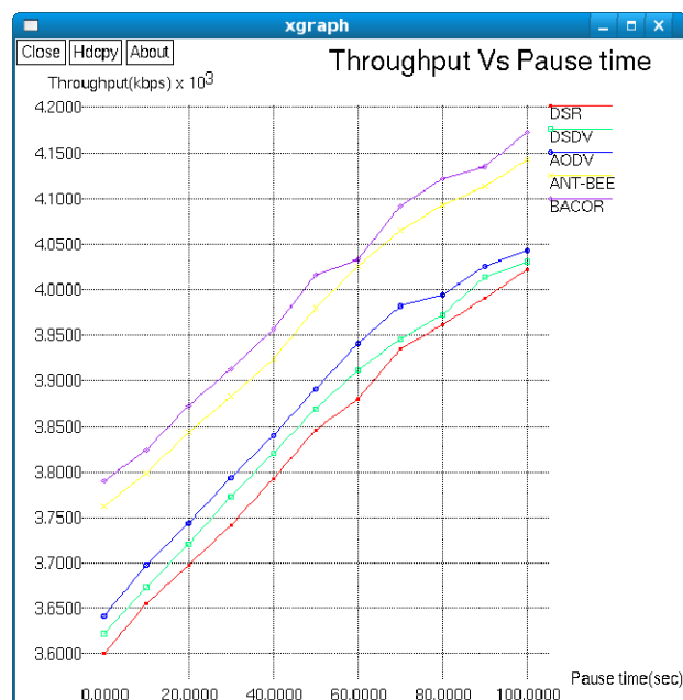
Figure7. Throughput Vs Pause Time
