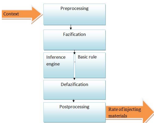
Figure 3 .Fuzzy controller
