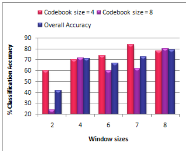
Figure 3: % classification accuracy for respective pixel window sizes
