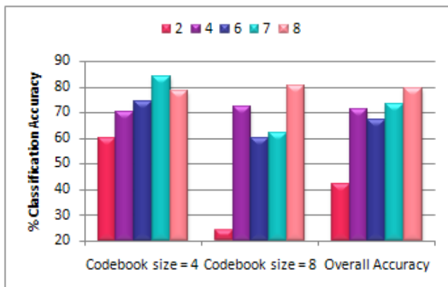
Figure 4: % classification accuracy for considered codebook sizes
