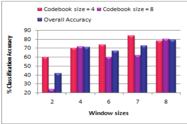
Figure 3: % classification accuracy for respective pixel window sizes
