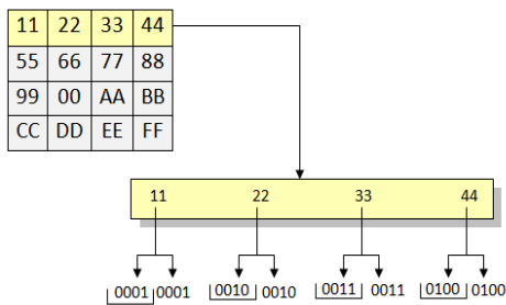
Fig. 2 Modified Sub Bytes
