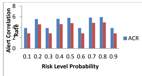
Fig.2 Alert Correlation Rate using ACR and UFP-GA
