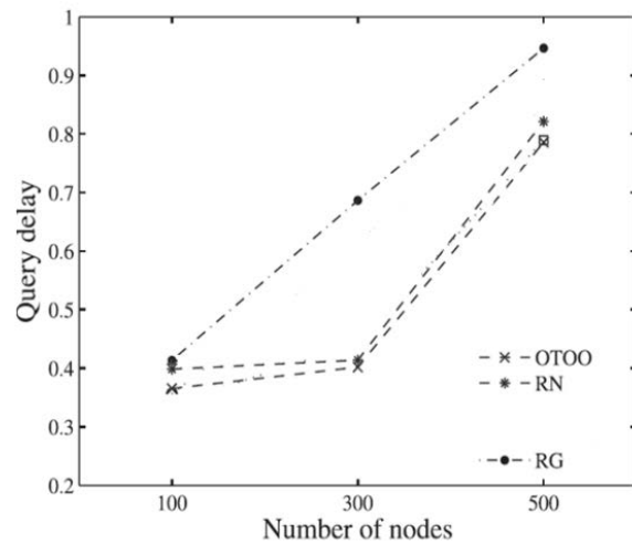
Fig.3 Query Delay
