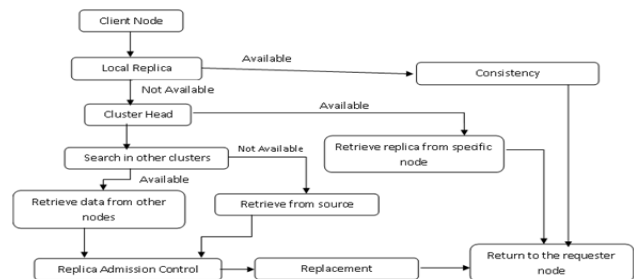
Fig.1 Replica Management Using Clustered Approach
