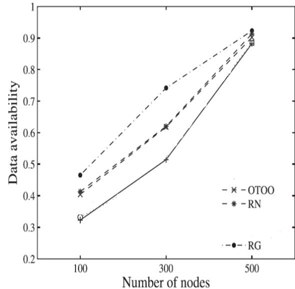
Fig.2 Data Availability
