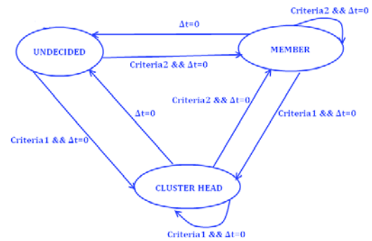
Fig. 2 Transitions between modes. (Criteria1: E_i \geq E ; Criteria2: E_i < E ).
