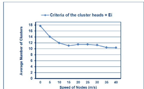
Fig. 4 Average number of clusters vs. speed of nodes.
