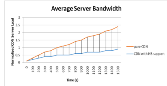
Fig8: HB Bandwidth Utilization
