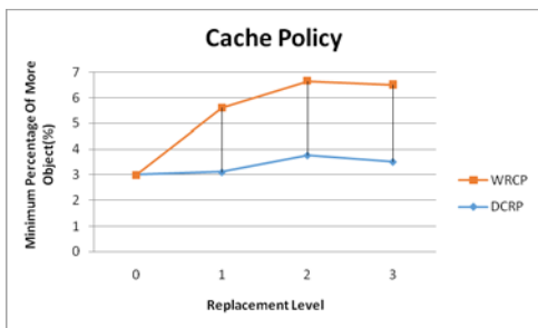
Fig6: Minimum percentage of more object allowed
