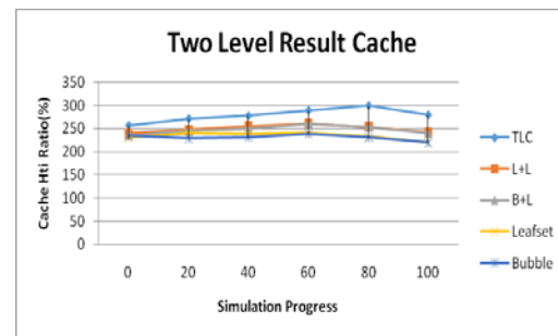
Fig2: Cache hit ratio (TLC)
