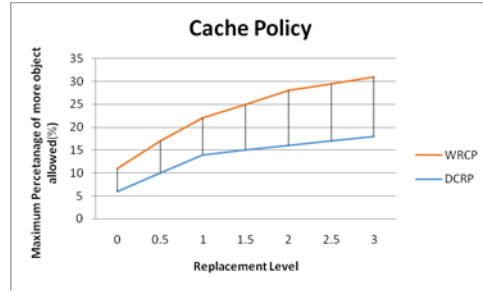
Fig7: Maximum percentage of more object allowed
