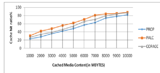
Fig:1 Cache hit ratio (PALC)
