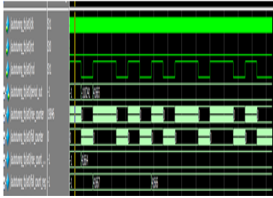
Figure 3: Auto tuning baud rate generator waveforms.
