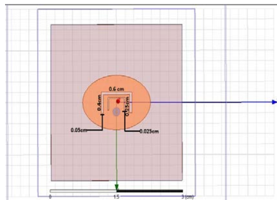
(3) Figure represents the closer view of the design
