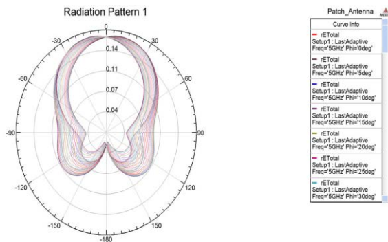
(6) Figure represents 2D gain total
