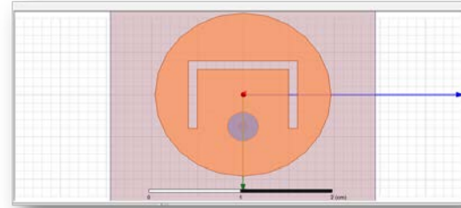
The design of elliptical patch antenna with single U-slot by using HFSS software is shown above in figure (1)
