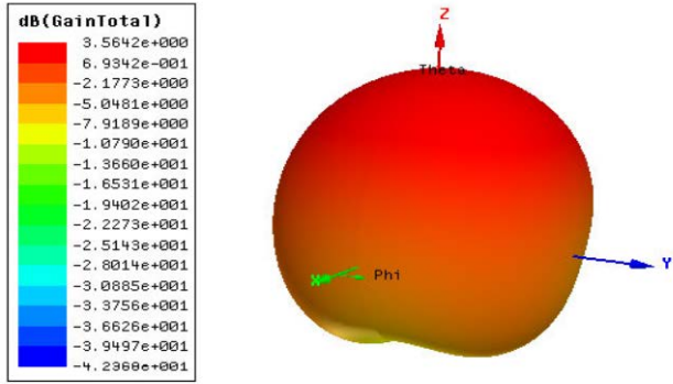
(9) Figure represents the 3D gain total
