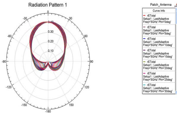
(10) Figure represents the Radiation pattern
