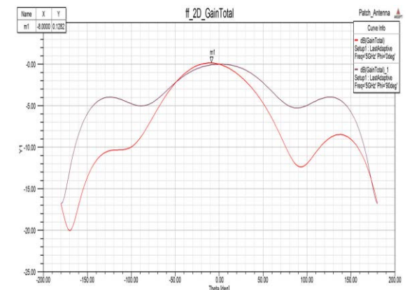
(7) Figure represents 2D gain total
