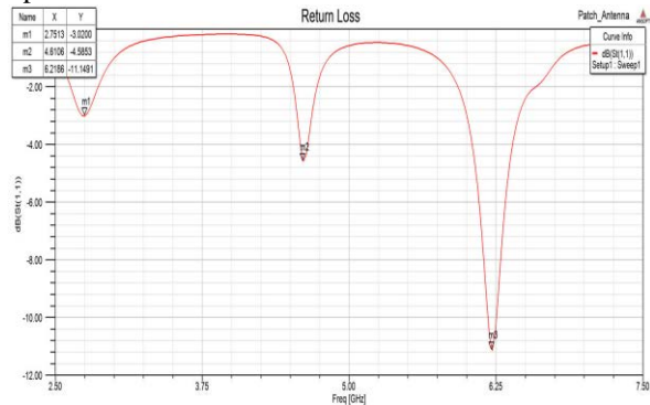
(8) Figure represents Return losses
