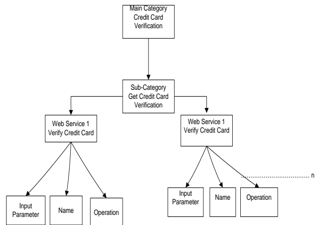
Figure 2: Ontological Arrangement of Web Services
