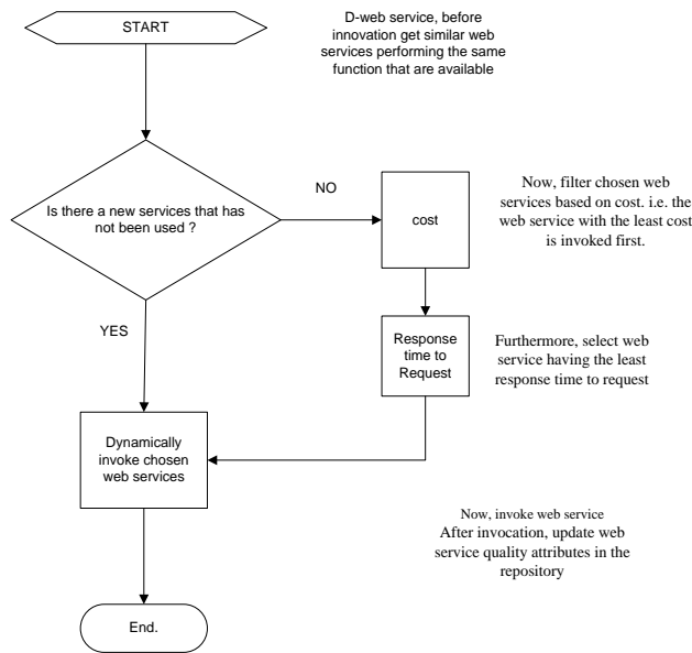
Figure 4 the web service selection algorithm
