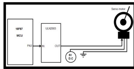
Figure 101: Servo motor interface
