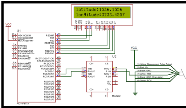
Figure 18: GPS to PIC interface
