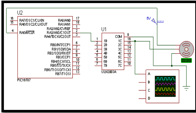
Figure 17: servo motor to PIC interface
