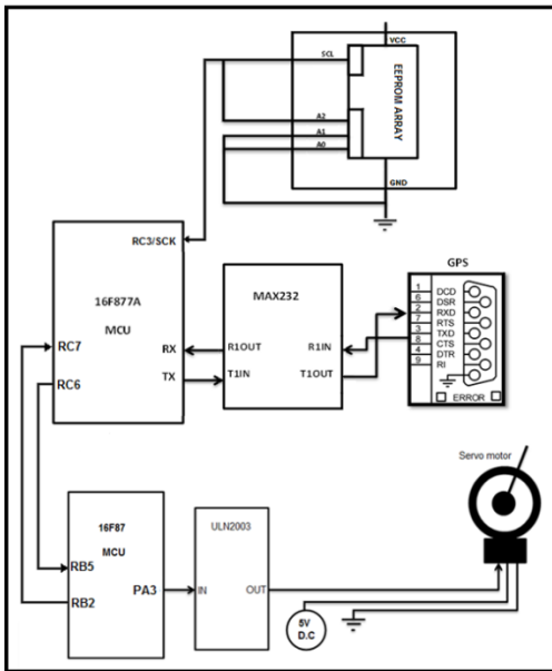
Figure 11: Servo motor simulation circuit
