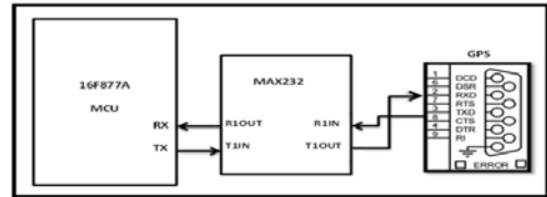
Figure 10: GPS interface
