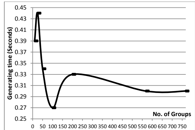
Figure 5.4- Graph for Generating time in second of FP-Growth.
