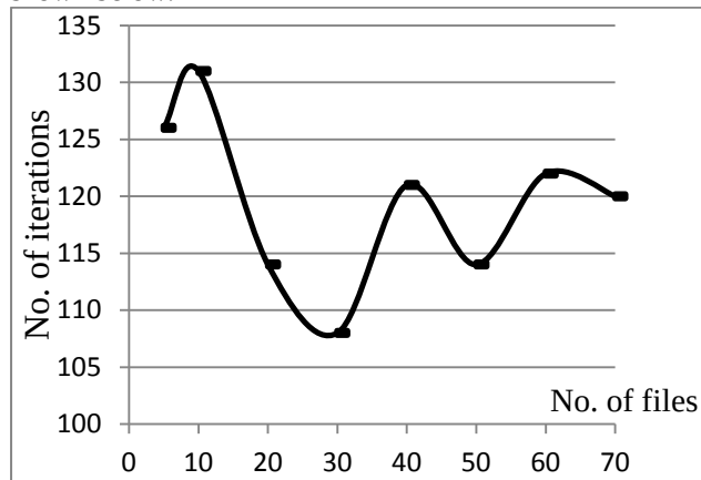
Figure 5.6 - No. of iterations for documents in clustering.
