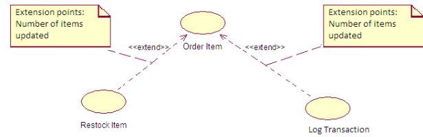
Fig. 12. The order in which Restock Item and Log Transaction will be inserted into Order Item is not deterministic, because they both reference the same extension point in this model. If the transaction must be logged before the item is restocked, Log Transaction must be inserted at an extension point located at a place defined earlier in the flow than the extension point Number of Items Updated.
