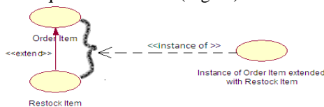
Fig. 4. The use-case instance to the right follows the description of the Order Item use case extended by the description of the Restock Item use case, as indicated by the hatching.
