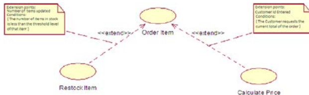
Fig.10. An extend relationship has a condition that states under what circumstances the extension is to take place. The condition can include references to information inside the system and to interactions between an actor and the system.
