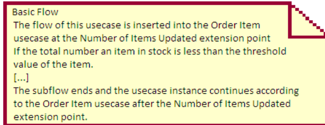
Fig. 11. The description of Restock Item includes a description of the extend relationship as a description of where and why the flow is added. The end of the flow description is also slightly affected by the extend relationship.
