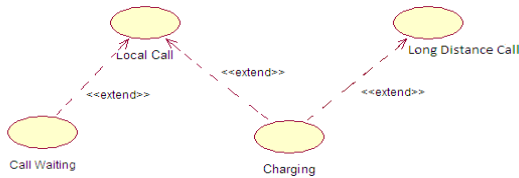
Fig. 8. One use case may extend several use cases, and several use cases may extend the same (base) use case.
