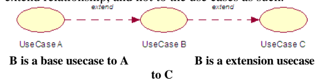
Figure 1. The terms base use case and extension use case are relative terms.
