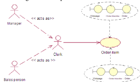
Fig. 2. Example of a Warehouse.
