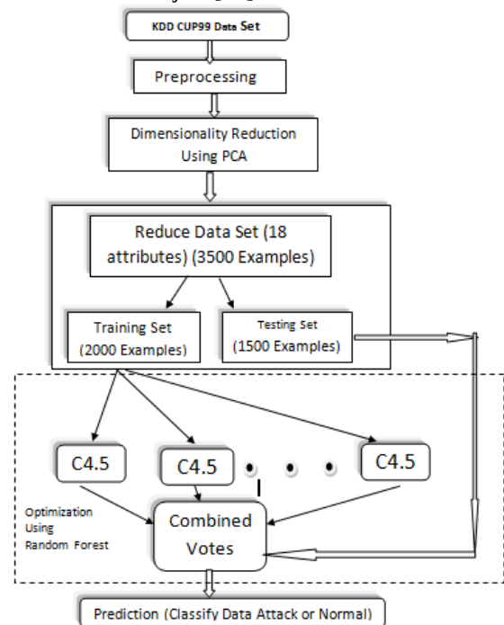
Fig.1 The Complete Proposed Model
