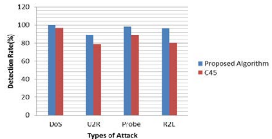
Fig. 4 Comparison of proposed algorithm with C4.5
