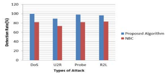
Fig. 3 Comparison of proposed algorithm with Naive Bayes Classifier
