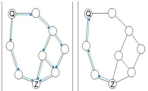
Figure 5: Ad hoc On Demand Distance Vector Routing
