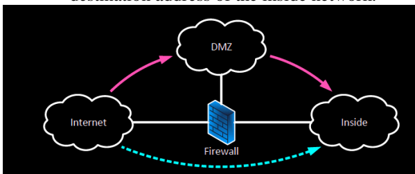
Figure 1.4.: Firewall Bypassing with RH0: the firewall would block a direct connection from the Internet to the inside network, but allows it through the DMZ.
