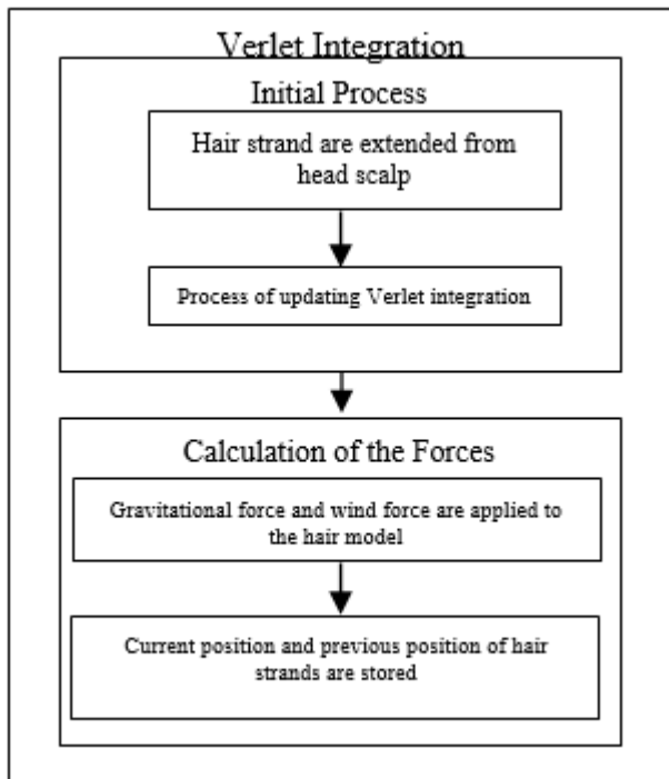
Fig. 6 Framework of implementation of Verlet integration
