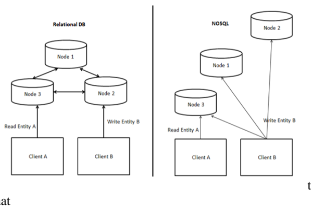
Fig. 5 Relational DB vs. NoSQL.
