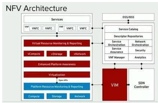
Fig. 4 Network Functions Virtualization Architecture Source: (Google.com, 2018)
