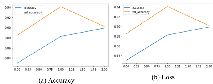
Fig.6 Impact of Early Stopping on Levenberg–Marquardt method
