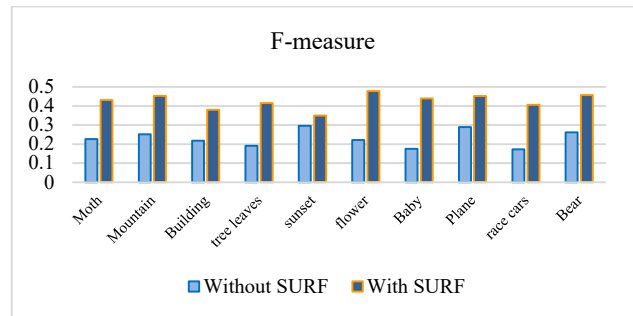
Figure 5: F-Measure Results
