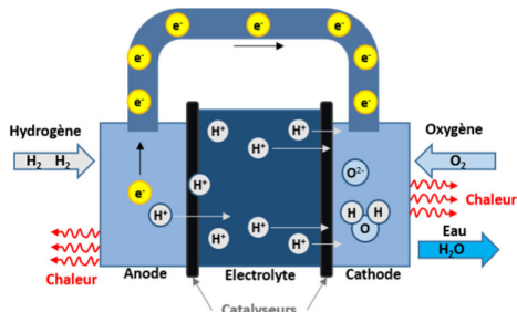
Fig 2: Fuel Cell Schematic
