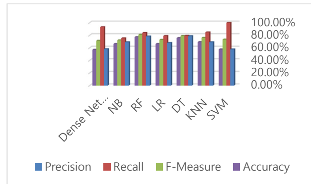
Figure 3: Average results of Precision, Recall, F-measure, Accuracy
