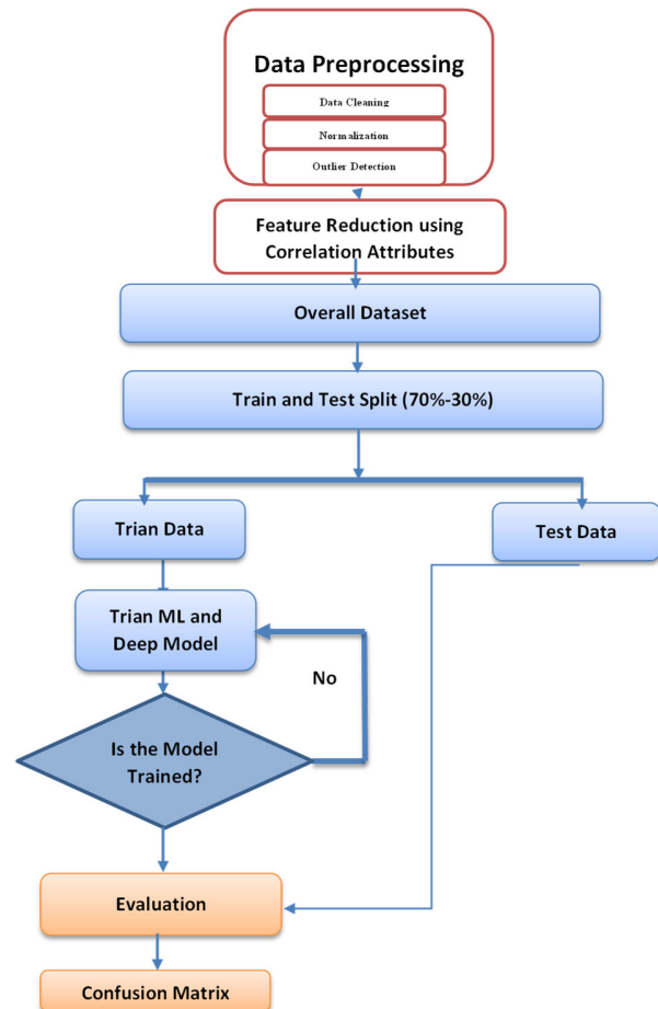
Figure 1: Proposed Approach
