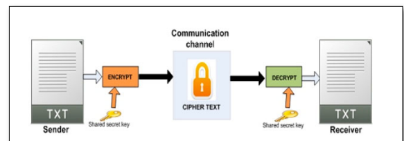
Fig. 2 Symmetric cryptography[6].
