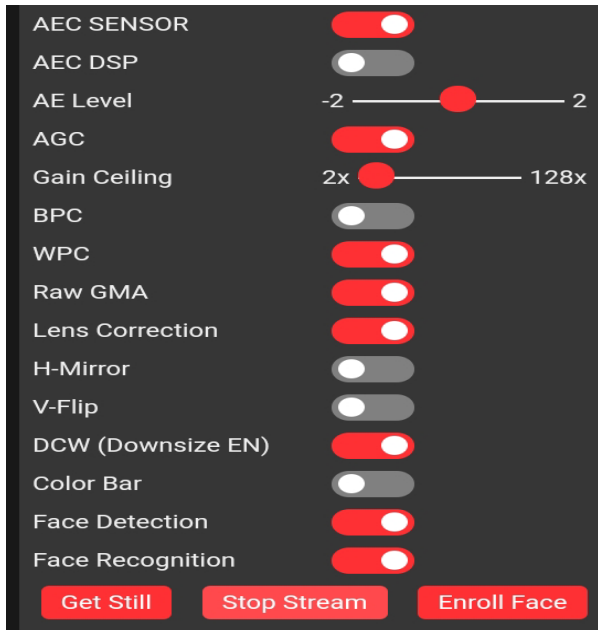
Fig. 9. : Camera feature
