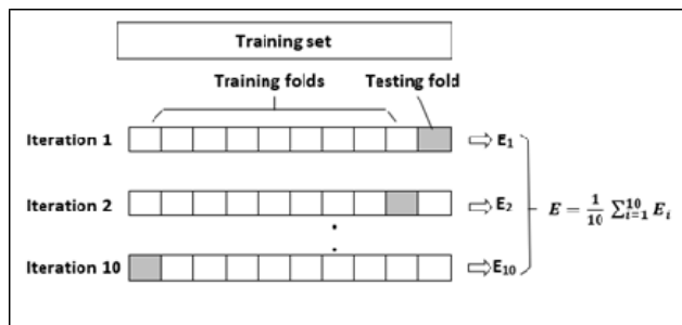
Fig. 2 10-folds cross-validation [19]
