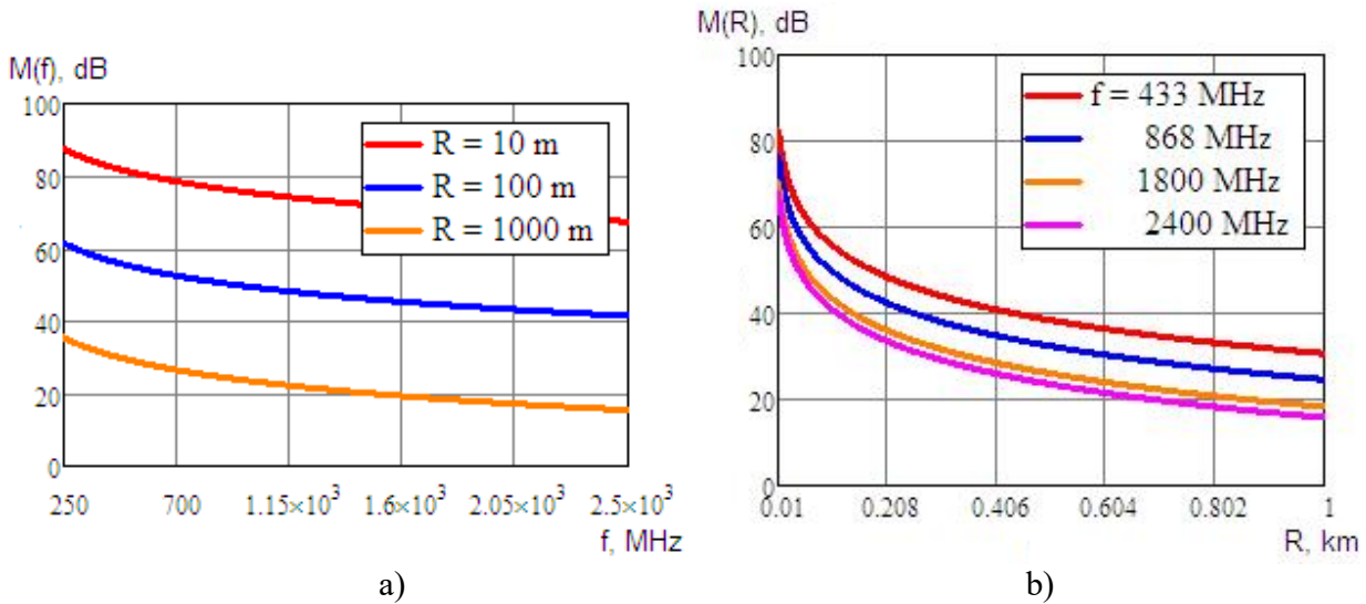
Figure 1-Dependence of the energy reserve of the communication channel during data transmission between UAVs on the carrier frequency of the transmitted radio signal (a) and the distance between the transmitting and receiving nodes of the communication network (b)
