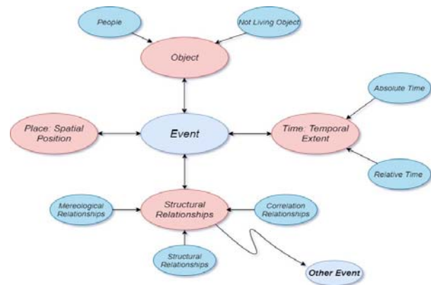
Fig 4. Event-Model-F ontology [8]
