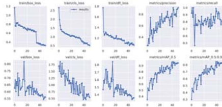
Fig.18 results for YOLO v9 epoch 100
