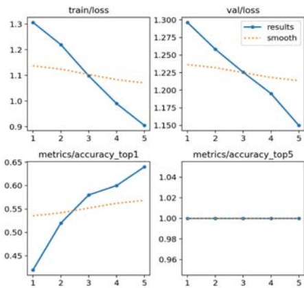
Fig. 3 Results for YOLO v8 epoch 5
