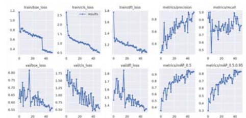
Fig. 16 Results for YOLO v9 epoch 50
