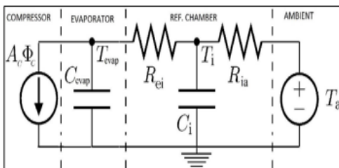
Figure 8. Refrigerator mode
