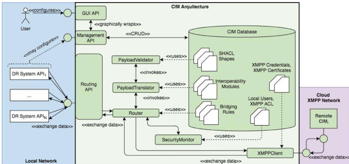
Fig. 2. CIM architecture.
