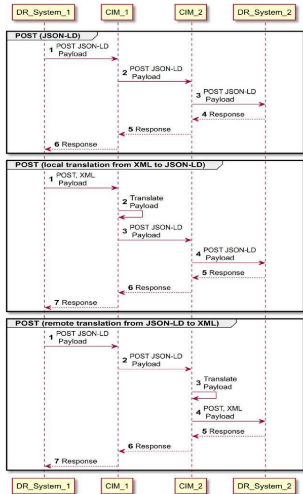
Fig. 6. Flows in experiment 1 for POST requests.
