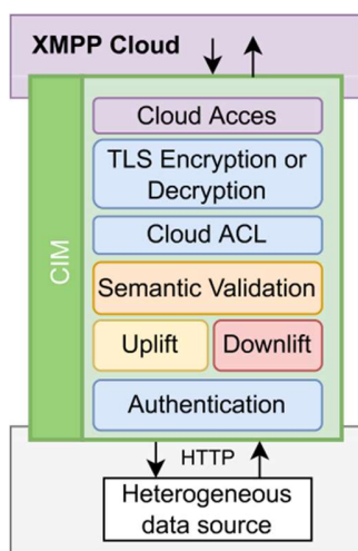
Fig. 1. CIM architecture.
