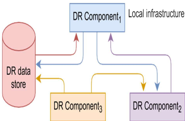
Fig. 3. A centralised DR system.
