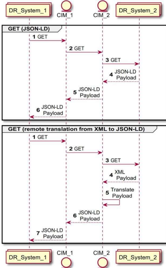
Fig. 5. Flows in experiment 1 for GET requests.
