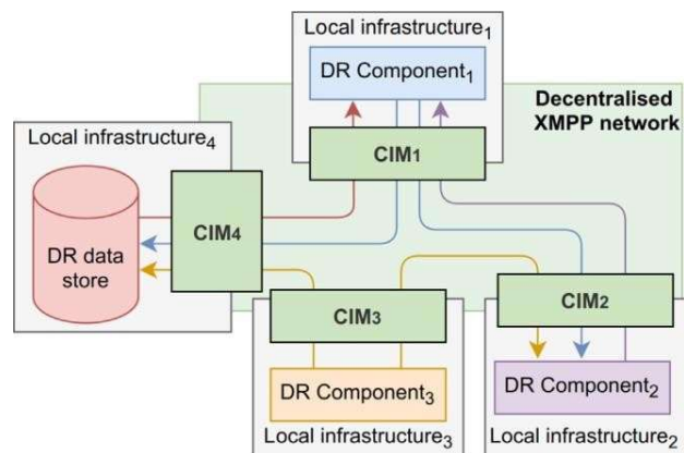
Fig. 4. A decentralised DR system using the CIM.
