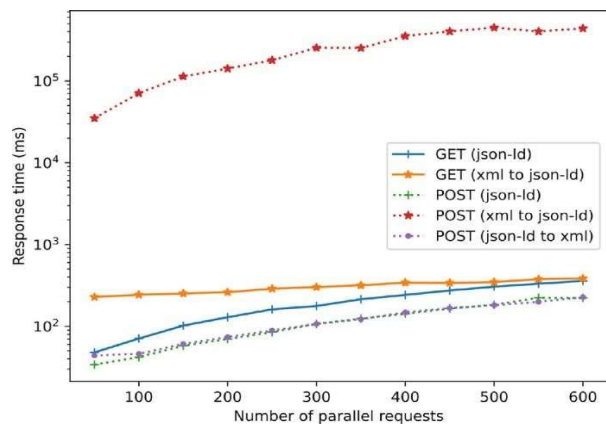
Fig. 7. Response times for scaling parallel requests.
