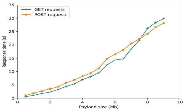
Fig. 8. Response times for scaling a payload size.
