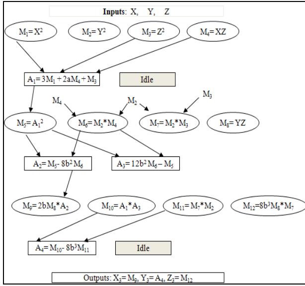
Figure 1: Hardware design for Montgomery ECC computations
