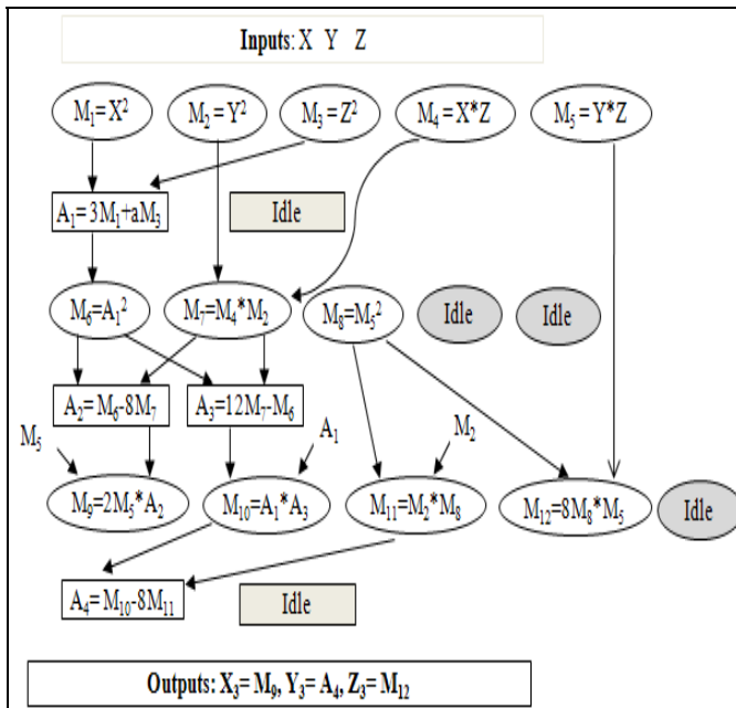
Figure 2: Hardware design for Weierstrass ECC computations
