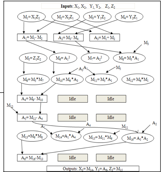
Figure 3: Hardware design for point addition computations
