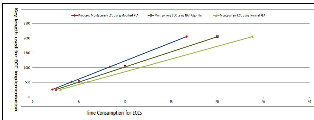
Figure 4: Comparison between performance levels for presented Montgomery ECC using different key lengths
