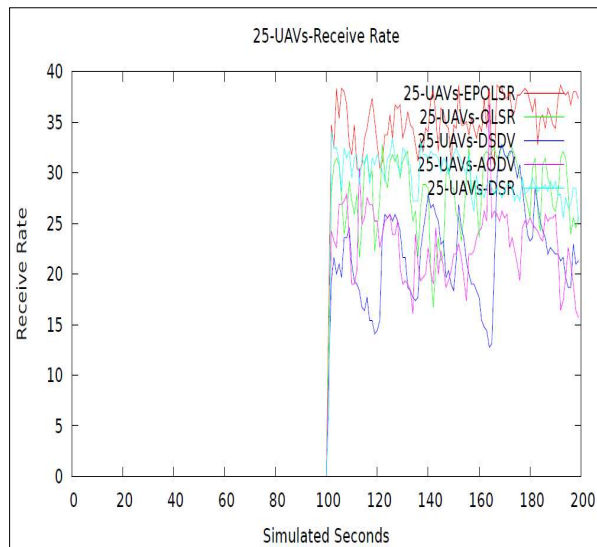
Figure. 10. 25-UAVs- Receive Rate (kbps) Using EP OLSR vs. OLSR, DSDV, AODV, and DSR
