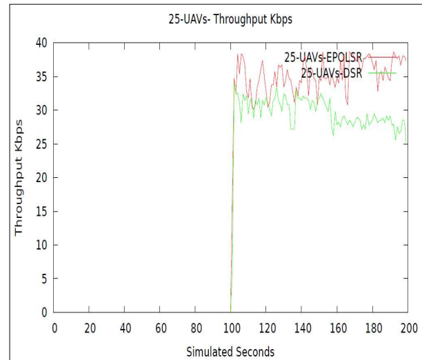
Figure. 19. 25-UAVs- throughput (kbps) Using EP OLSR vs DSR
