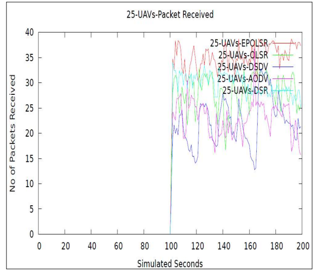
Figure. 15. 25-UAVs- No of Packets Received (kbps) Using EP OLSR vs. OLSR, DSDV, AODV, and DSR
