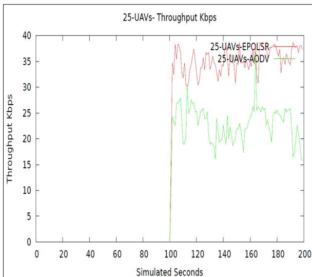
Figure. 18. 25-UAVs- throughput (kbps) Using EP OLSR vs AODV
