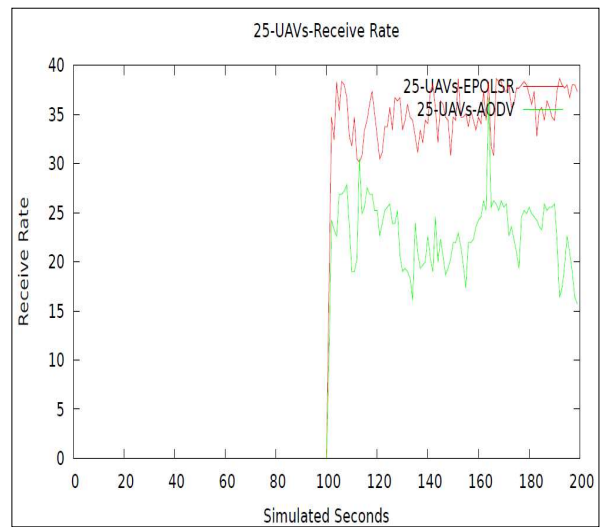
Figure. 8. 25-UAVs- Receive Rate (kbps) Using EP OLSR vs. AODV
