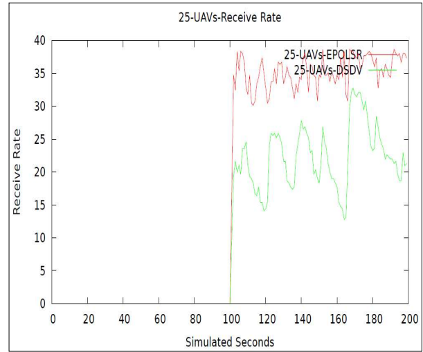
Figure. 7. 25-UAVs- Receive Rate (kbps) Using EP OLSR vs. DSDV
