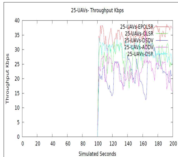
Figure. 20. 25-UAVs- throughput (kbps) Using EP OLSR vs OLSR, DSDV, AODV, and DSR
