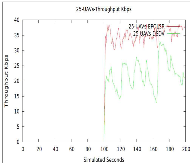
Figure. 17. 25-UAVs- throughput (kbps) Using EP OLSR vs. DSDV
