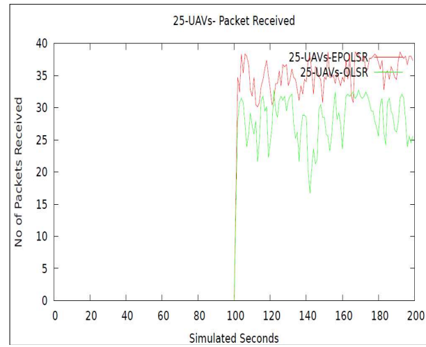
Figure. 11. 25-UAVs- No of Packet Received (kbps) Using EP OLSR vs. OLSR
