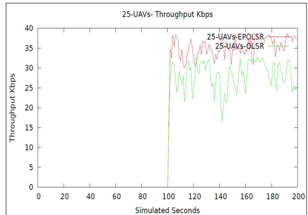
Figure. 16. 25-UAVs- throughput (kbps) Using EP OLSR vs. OLSR
