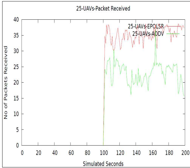
Figure. 13. 25-UAVs- No of Packet Received (kbps) Using EP OLSR vs. AODV
