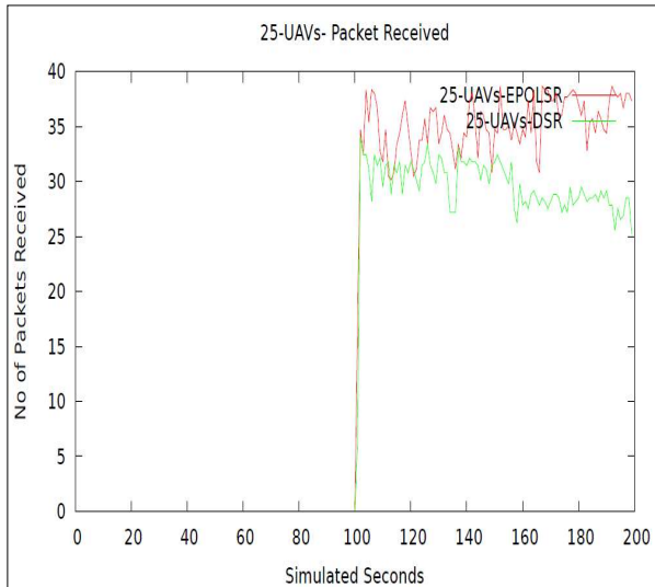
Fig. 14. 25-UAVs- No of Packet Received (kbps) Using EP OLSR vs. DSR
