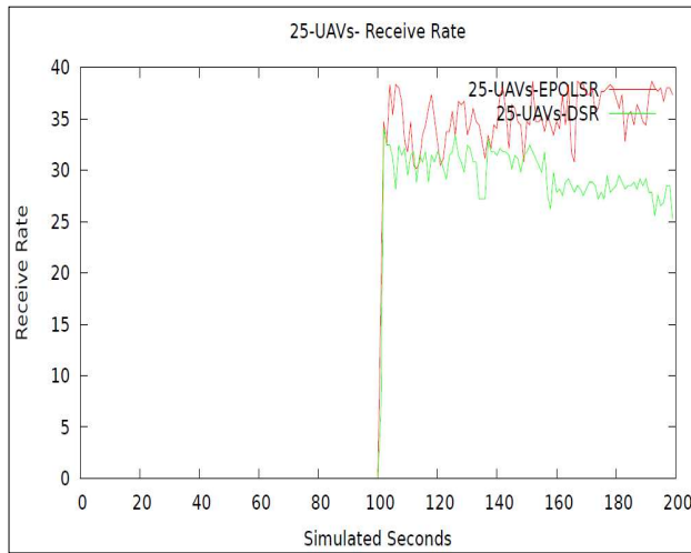
Figure. 9. 25-UAVs- Receive Rate (kbps) Using EP OLSR vs. DSR
