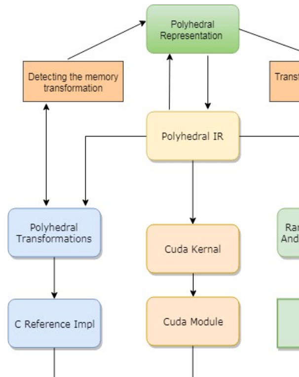
Figure.3. Modified proposed taxonomy for parallel process
