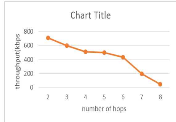
Fig. 1 : TCP connection throughput
