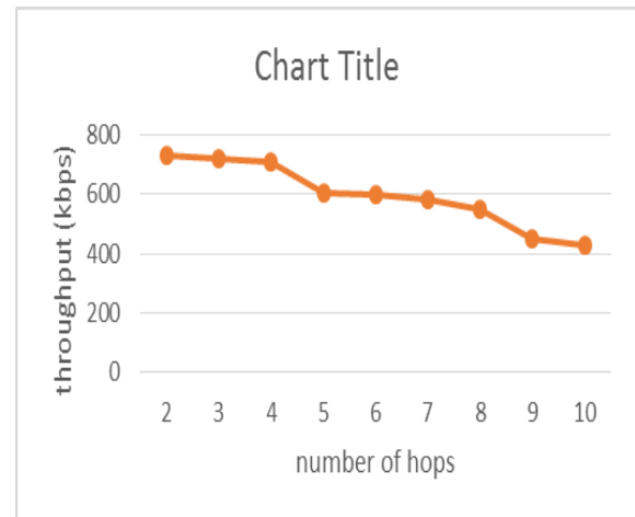
Fig. 2: throughput of TCP connection according to proposed model
