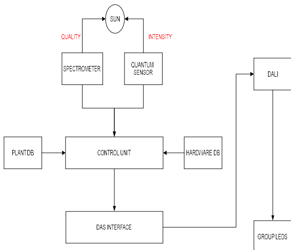
Figure 3. DAS block diagram.
