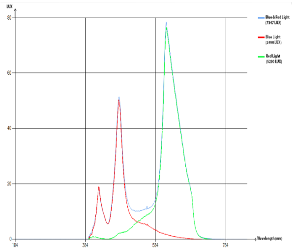
Figure 5. Experimental results for LED.
