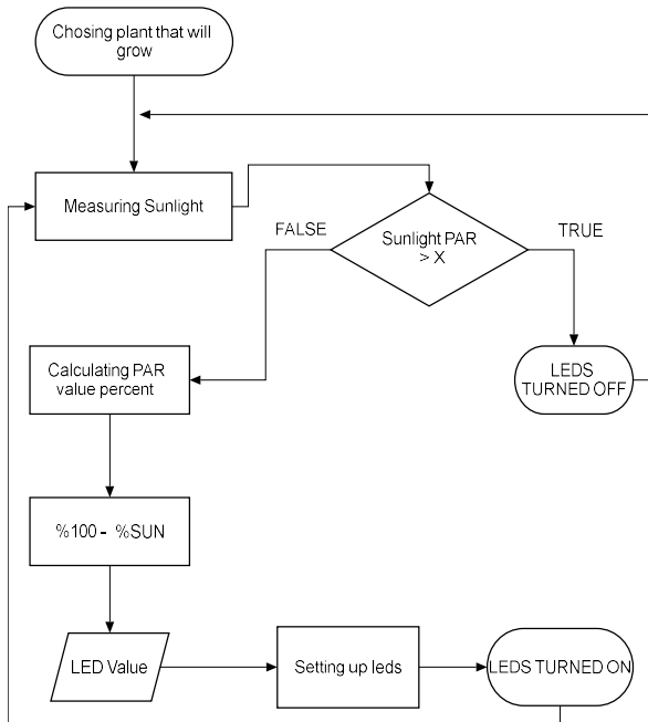
Figure 2. Flowcharts of the DAS algorithm.
