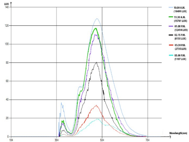
Figure 4. Experimental results for SUNLIGHT.
