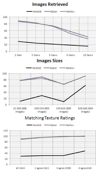
Figure. 8: investigation of the retrieval algorithm
